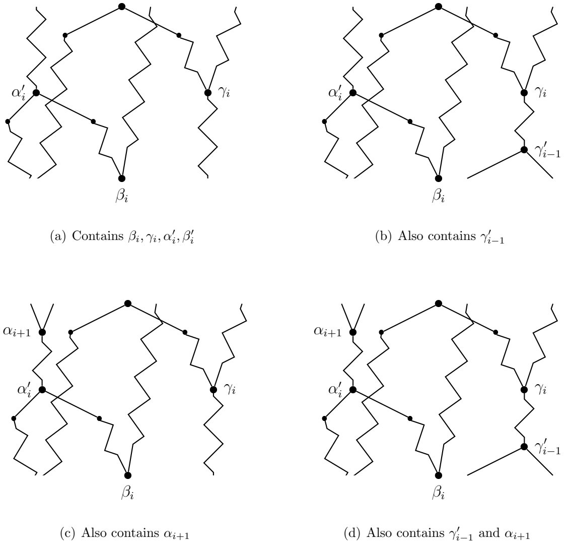
Figure 2.4: Points in [\beta_i, \beta'_i] — 4 possible cases
